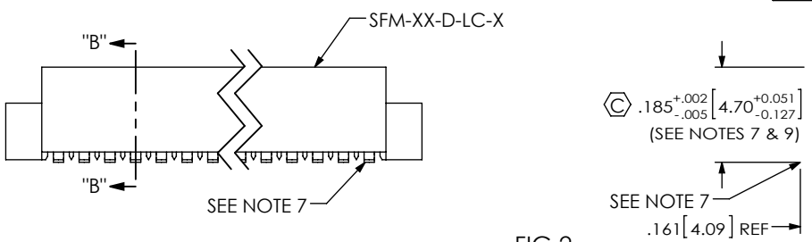
FIG 2 -X2: SURFACE MOUNT (SAME AS FIG 1, DIFFERENT AS SHOWN)
