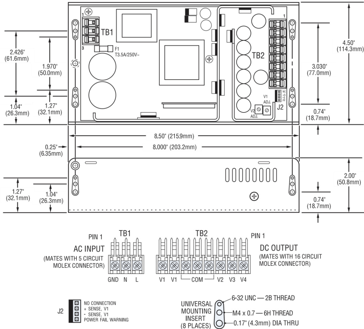
Figure-1 - Mechanical Drawing
