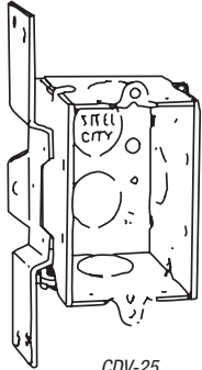
CDV-25 "CV" bracket recessed 1/4"
