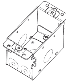
Combination 1/2" & 3/4" Knockout
