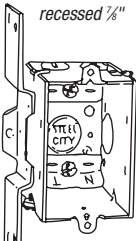
CWNV-25 "CV" bracket recessed 3/8"
