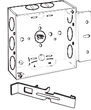
52151 MS N* "MS" bracket for 1½", 2¼", 3½", 4"
