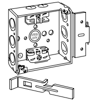
52151 MS X* "MS" bracket for 1½", 2¼", 3½", 4" metal studs
