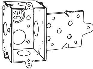
804 S "S" bracket recessed 1/4"
