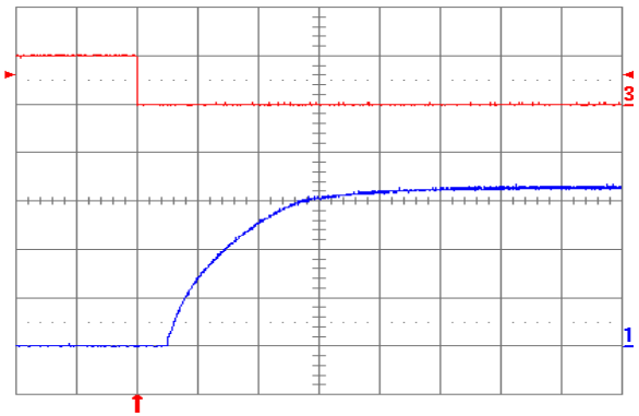
Fig. 3.3V.8: Turn-on transient at full rated load current (resistive) plus 10,000 µF at V_{in} = 48\text{ V} , triggered via ON/OFF pin. Top trace: ON/OFF signal (5 V/div.). Bottom trace: Output voltage (1 V/div.). Time scale: 1 ms/div.
