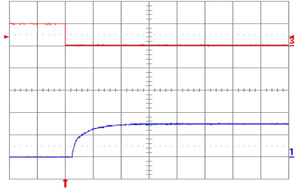
Fig. 1.5V.8: Turn-on transient at full rated load current (resistive) plus 10,000 µF at V_{in} = 48\text{ V} , triggered via ON/OFF pin. Top trace: ON/OFF signal (5 V/div.). Bottom trace: Output voltage (1 V/div.). Time scale: 2 ms/div.
