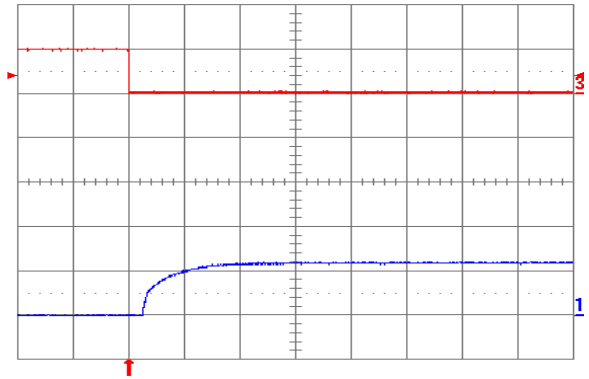
Fig. 1.2V.8: Turn-on transient at full rated load current (resistive) plus 10,000 µF at V_{in} = 48\text{ V} , triggered via ON/OFF pin. Top trace: ON/OFF signal (5 V/div.). Bottom trace: Output voltage (1 V/div.). Time scale: 2 ms/div.
