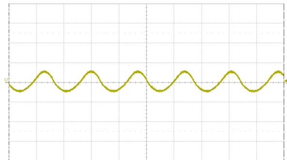
Fig. 16: Input reflected ripple current, i_s (50 mA/div.), measured through 10 \mu\text{H} at the source at full rated load current and V_{in} = 48 \text{ V} . Refer to Fig. 14 for test setup. Time scale: 2 \mu\text{s}/\text{div} .
