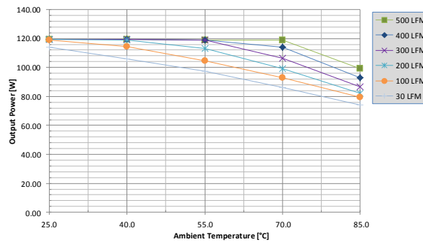
Fig. 4: Power derating vs. ambient air temperature and airflow rates for UIE48T36033 converter w/o baseplate mounted vertically with air flowing from pin 3 to pin 1, MOSFET temperature \leq 125^{\circ}\text{C} , V_{in}=48\text{V}
