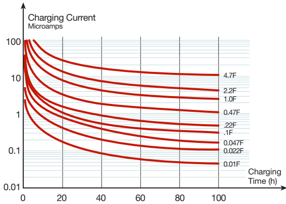
Figure 50. LX Series - 5 Volt Charge
