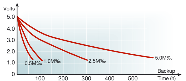
Figure 14. 0.22F – LC, LK, LT, LX, LJ, LM Series
