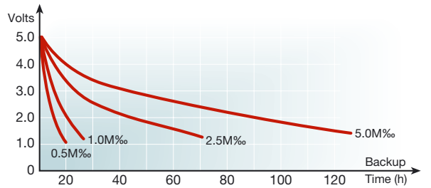
Figure 10. 0.047F – LC, LK, LT, LX, LJ, LM Series
