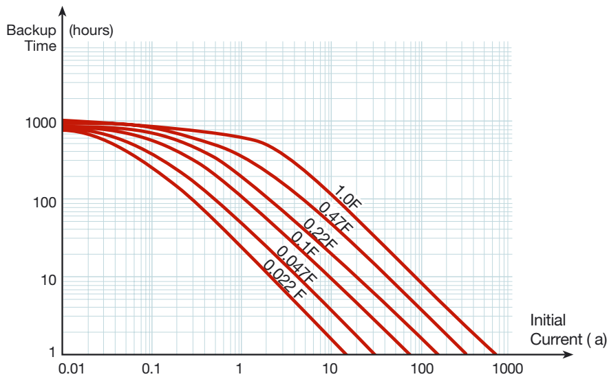
Figure 5. Minimum Backup Time Versus Initial Current for CMOS RAM Applications Using Maxcap DLC LP and LF Series from 5 to 2 Volts at 25°C
