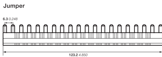
Jumper bar CR-S
