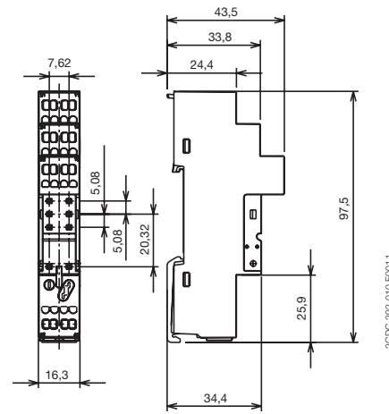
CR-PLC - spring connection
