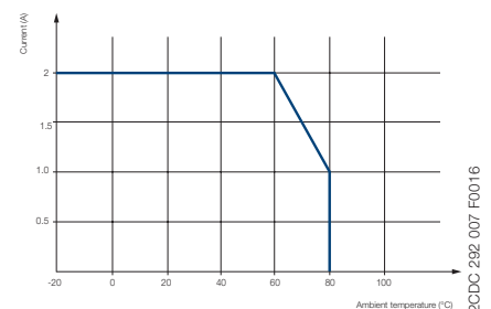
Derating curve Triac output
