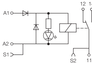
RB(R)121P(G)-5VDC/12VDC
