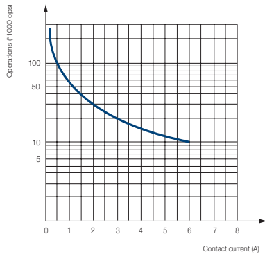
Endurance curve
