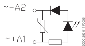
CR-P/M 62C, CR-P/M 92C, CR-P/M 62D, CR-P/M 62DV, CR-P/M 62V, CR-P/M 62CV, CR-P/M 92CV
