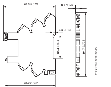
Spring socket for CR-S range interface relays
