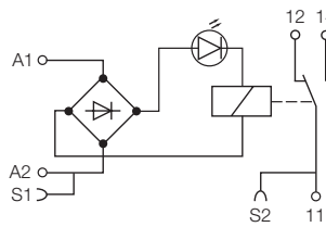
RB(R)121(G)-48-60VUC/ 115VUC/230VUC/60-230VUC
