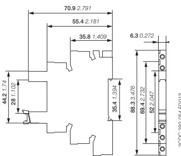
Screw socket for CR-S range interface relays
