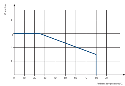
Derating curve MOS-FET output
